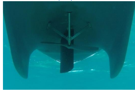
Keels, shaft, propeller & rudder
